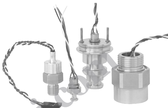
Possible versions of the pressure transducer TTF-1 (previous model 881.09.5295)
